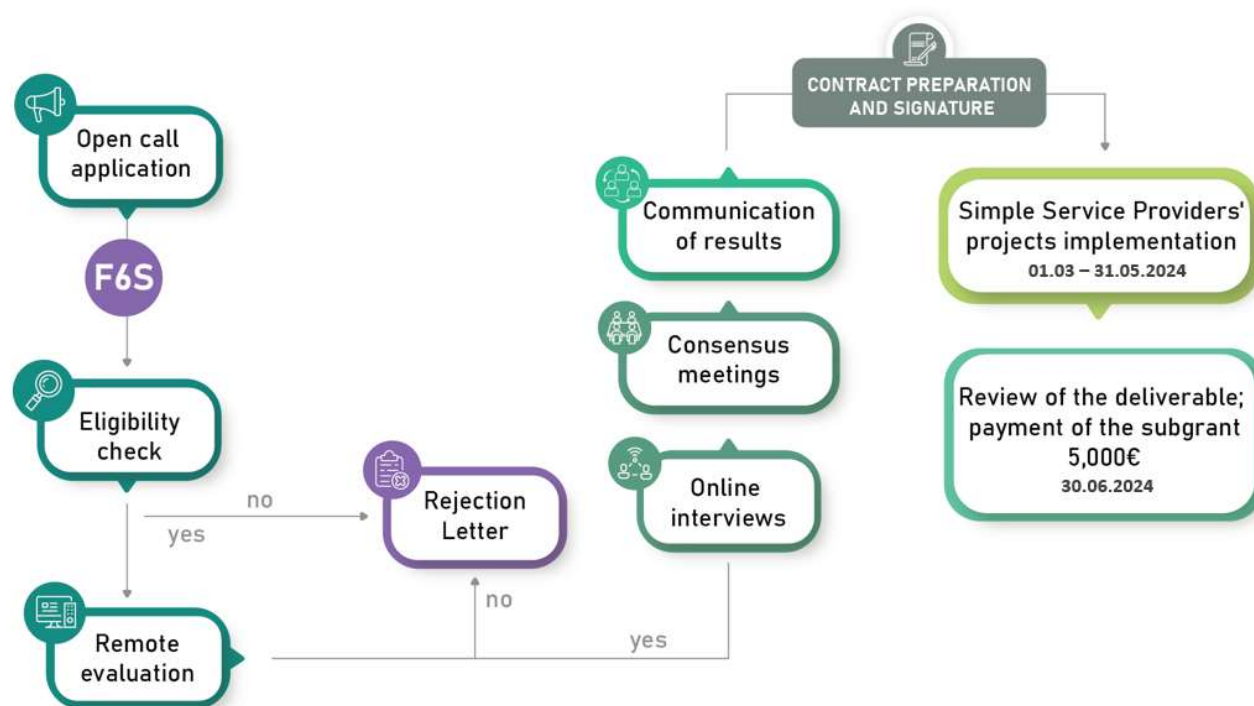
Figure 2 Open Call for Regional Demonstrators funnel – Simple Service Providers
